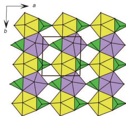
Figure 2. Section of a uranium silicate sheet in 1 . The purple and yellow polyhedra represent \text{U}(2)^{\text{V}}\text{O}_7 and \text{U}(3)^{\text{V/O}}\text{O}_7 pentagonal bipyramids, respectively. Silicate tetrahedra are in green.
